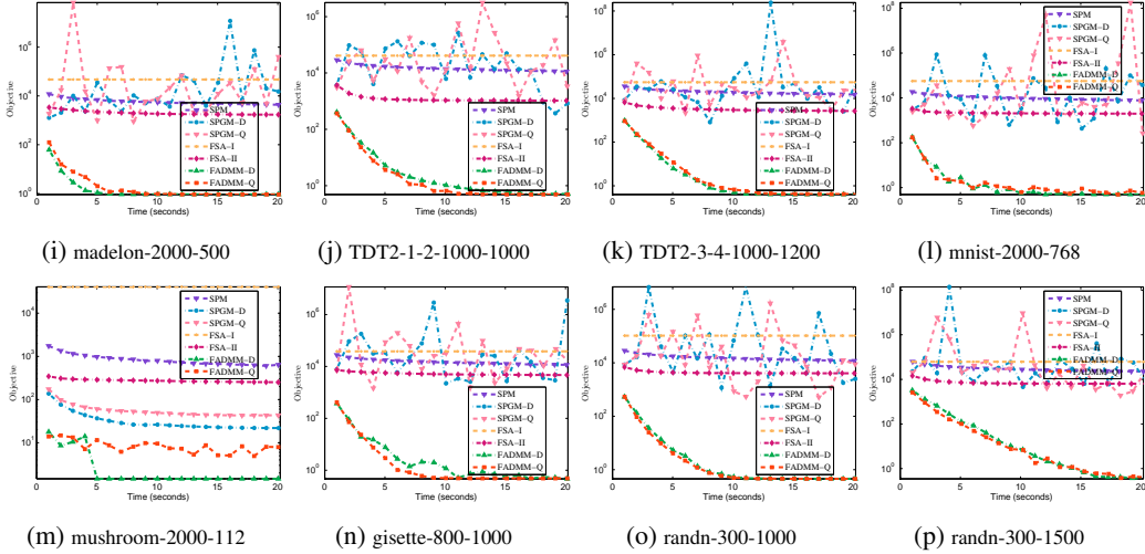
Figure 2: Results on sparse FDA on different datasets with \rho = 1000 .
