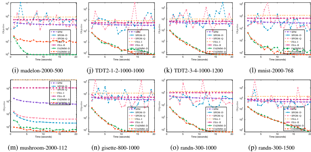
Figure 4: Experimental results on sparse FDA on different datasets with \rho = 10000 .
